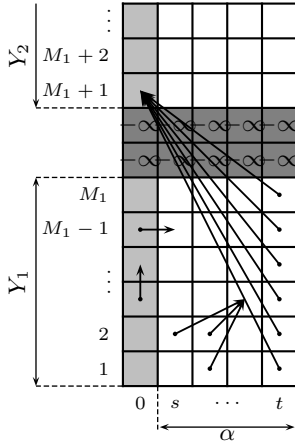
Figure 2: Illustration of the modifications of the thumbnailing algorithm for an excerpt of the similarity matrix \mathcal{S}(m, n) for n = [s : t] and m = [1 : M] corresponding to the subsequence \alpha = [s : t] .
