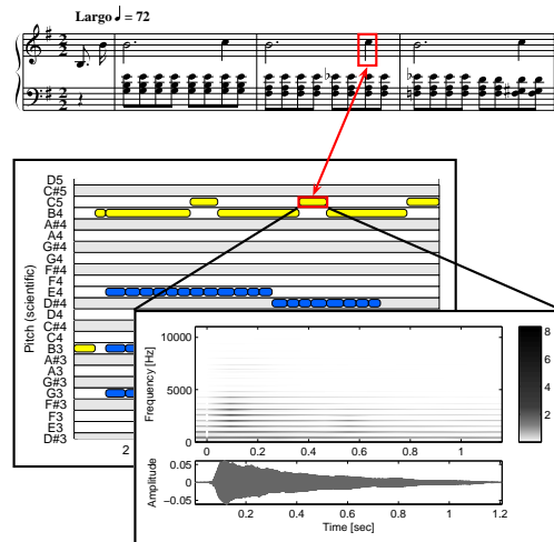
Figure 3: Top: Score of the first three measures of Op. 28 No. 4 by Frédéric Chopin. Bottom: Our user interface showing the corresponding part in an audio recording of the piece. Each note-wise audio event can be accessed separately.
