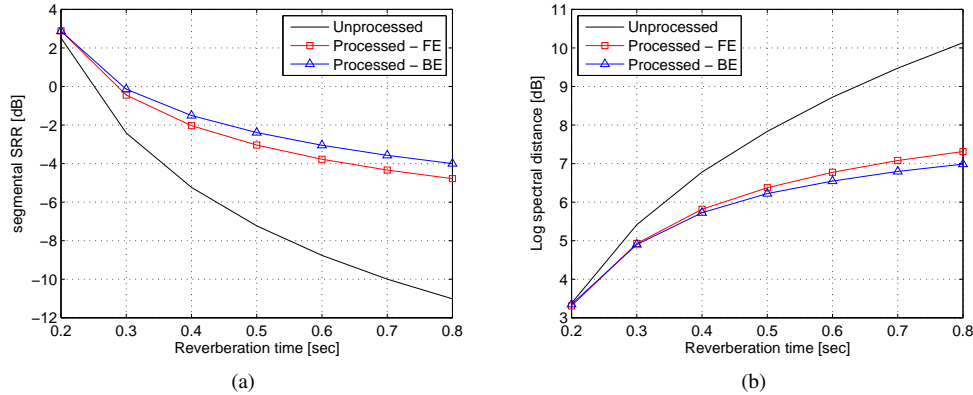
Fig. 2. Results of (a) segmental signal to reverberation ratio and (b) log spectral distance for the reverberant speech signals, processed signals using the forward estimator (FE) and processed signals using the backward estimator (BE) using different reverberation times.
