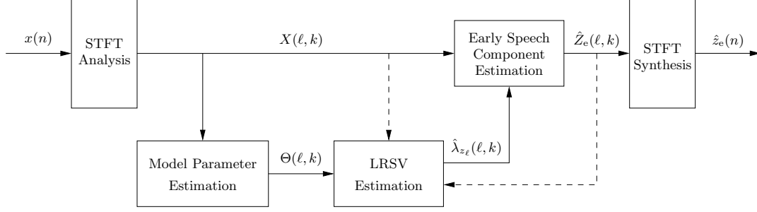
Fig. 1. Block diagram of the complete reverberation suppression system, which consists of a STFT analysis block, model parameter estimator, late reverberant spectral variance (LRSV) estimator, early speech component estimator, and STFT synthesis block.
